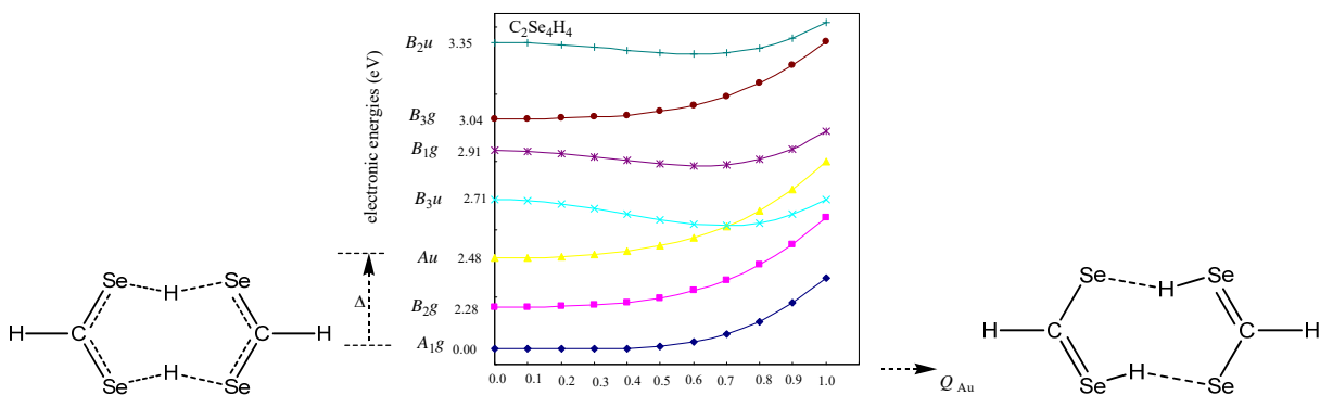
Figure 9: the calculated primary energy levels (the basic state and excited state A_u ) in the analog containing Se atom of methanoic acid dimer and their changes due to the PJTE (second state)
