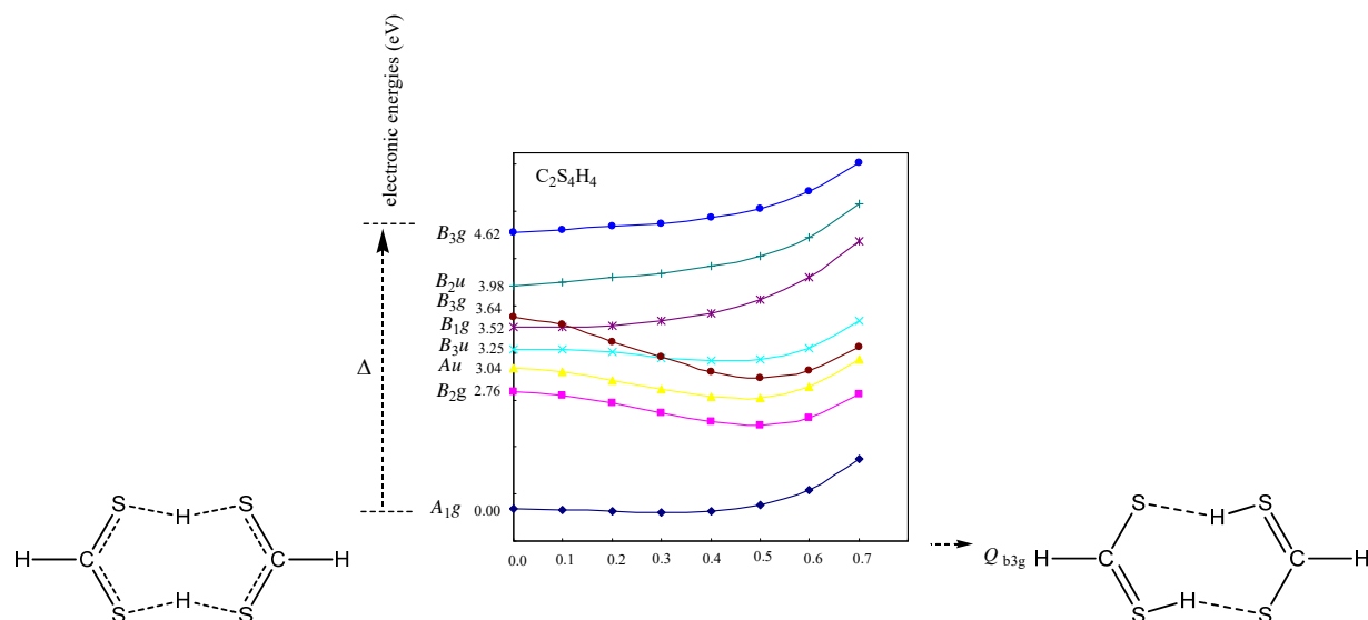
Figure 5: the calculated primary energy levels (the basic state and excited state B_{3g} ) in the analog containing S atom of methanoic acid dimer and their changes due to the PJTE (first state)
