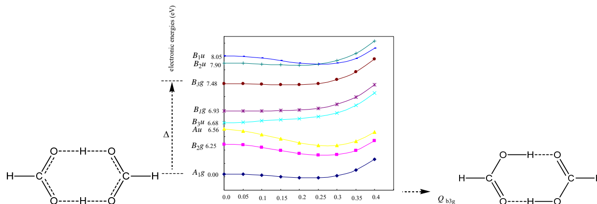
Figure 3: the calculated primary energy level (the basic and excited states) in the methanoic acid dimer and their distortions due to the PJTE
