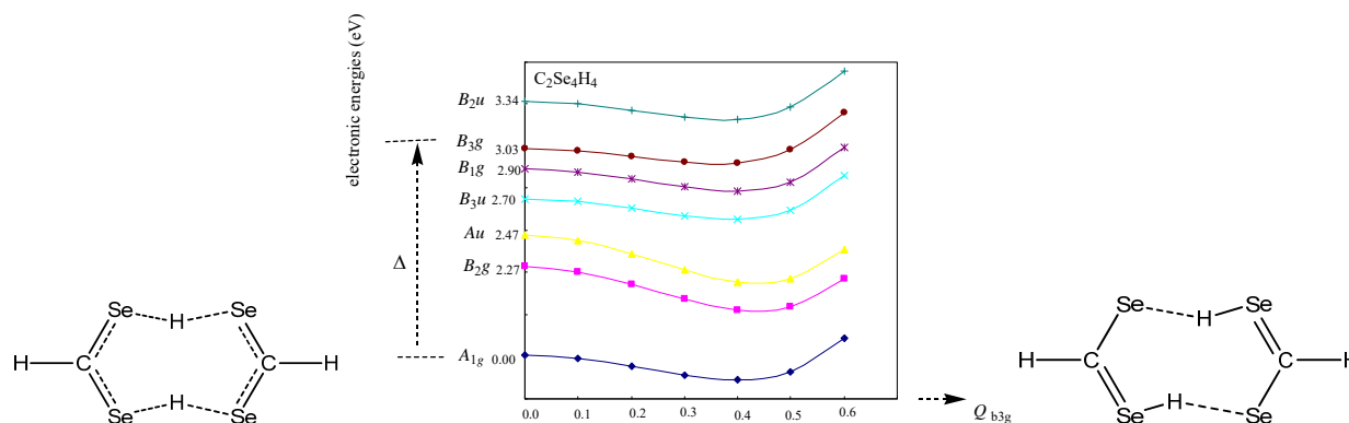
Figure 8: the calculated primary energy levels (the basic state and excited state B_{3g} ) in the analog containing Se atom of methanoic acid dimer and their changes due to the PJTE (first state)
