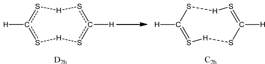
Figure 4: the change in the formation with the symmetry D_{2h} for the analog with S atoms in the methanoic acid dimer in the form of ( D_{2h} \rightarrow C_{2h} ) C_{2h} by the use of calculations in the theoretical level B3LYP.6-311++G**
