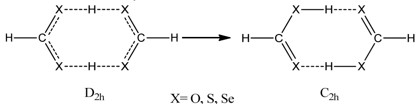
Figure 1: the transformation of the formation with the D_{2h} symmetry in dimeric methanoic acid and the analog containing S and Se atoms into the formation C_{2h} ( D_{2h} \rightarrow C_{2h} ) by the use of calculations at the theoretical level B3LYP/6-311++G** ( X=O, S, Se ).
