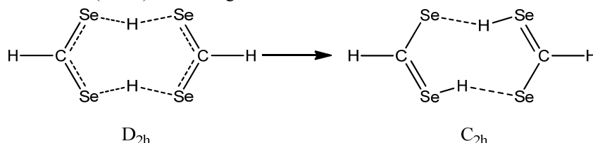
Figure 7: the change in the formation with the symmetry D_{2h} for the analog with Se atoms in the methanoic acid dimer in the form of ( D_{2h} \rightarrow C_{2h} ) C_{2h} by the use of calculations in the theoretical level B3LYP.6-311++G**
