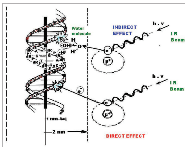
Figure 1: Scheme that represents (above) the indirect damage, by adding a radical \cdot\text{OH} to a nitrogenous base of a DNA strand. And below, the direct damage by the action of a photon or an electron torn from the surrounding material and impacting the DNA like a projectile, breaking the covalent bonds of a strand. Adapted from Giaccia and Cols
